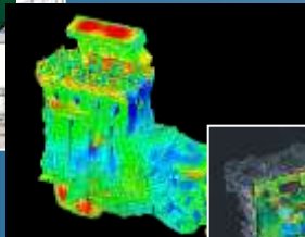
AVL-EXCITE
